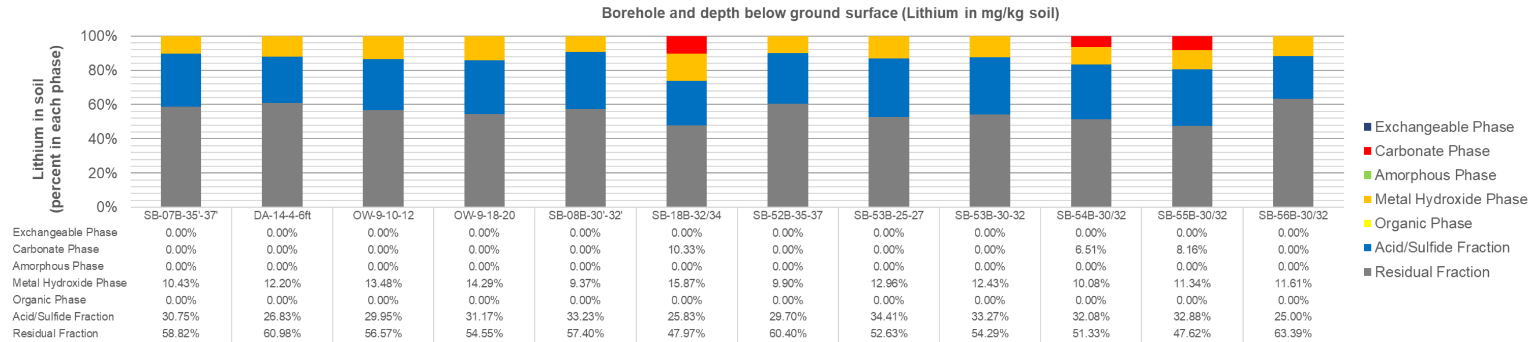
Borehole and depth below ground surface (Lithium in percent of total)
